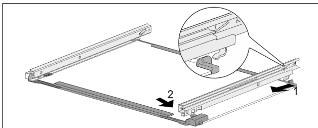
Fig. 42 Glass shelf with rails
